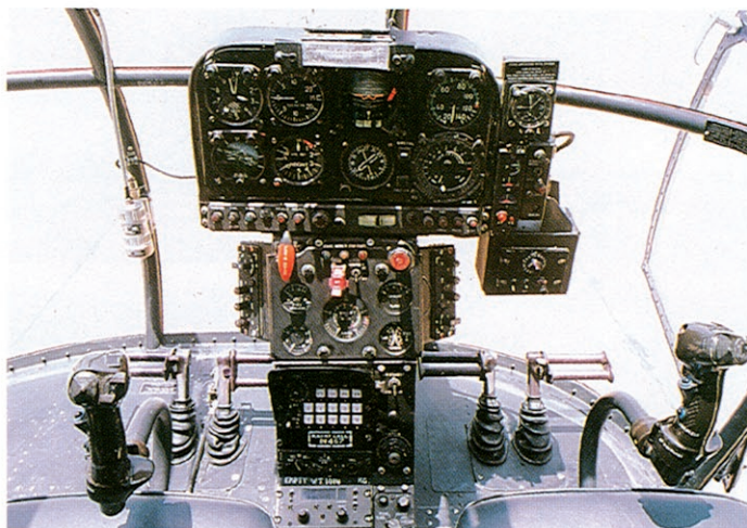
Electrical artificial horizon 4286 V8
