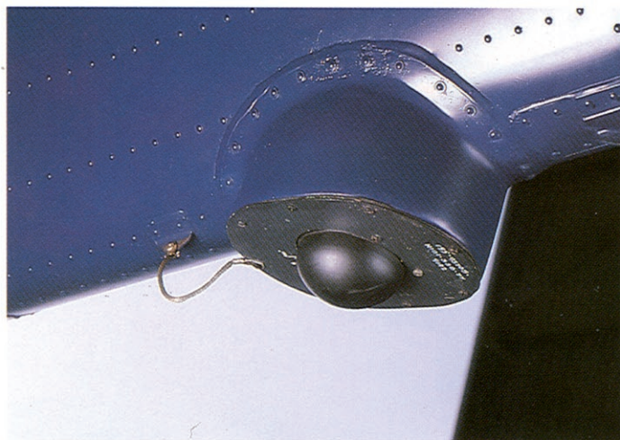
Flux valve for gyromagnetic compass CG-512-3
