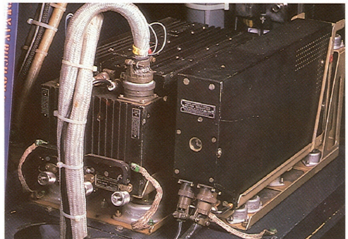
Automatic direction finder ARC 610A and communication system V/UHF type VUC-201A
