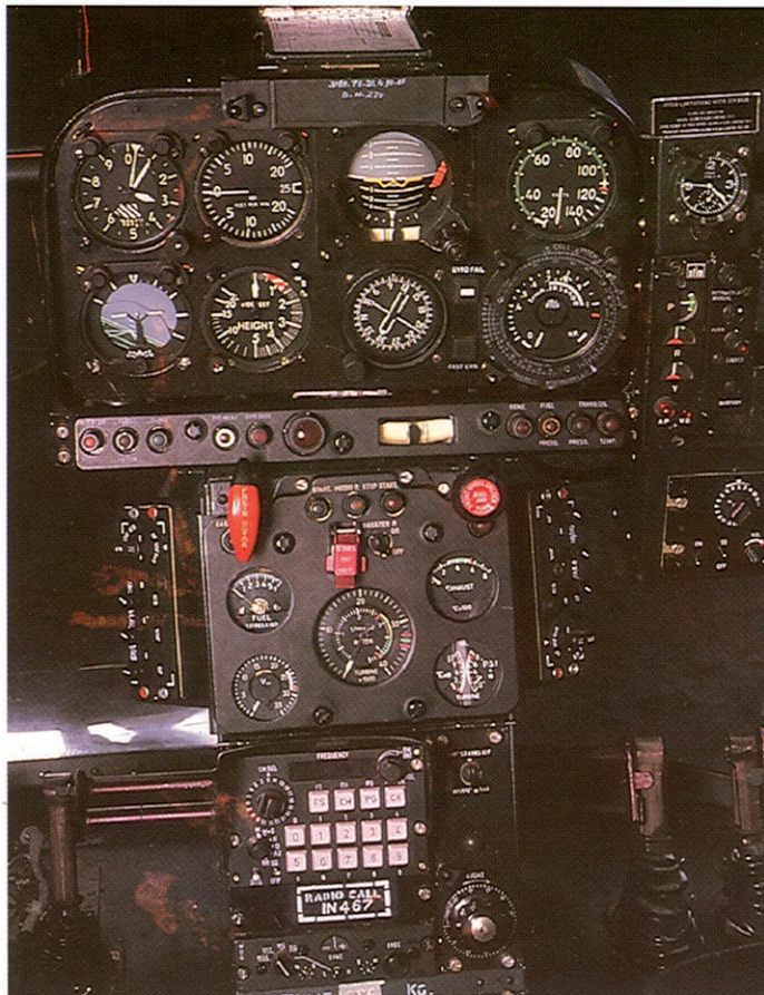
Automatic direction finder ARC 610A and communication system V/UHF type VUC-201A
