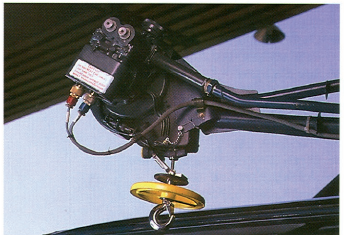
Rescue hoist
